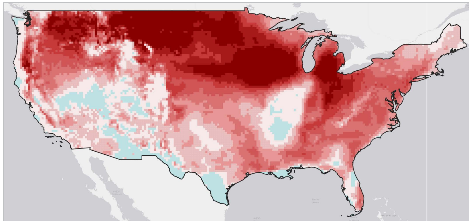
2050 days with maximum temperatures over 95F in 2050: Differences between CMIP6 and CMIP5
