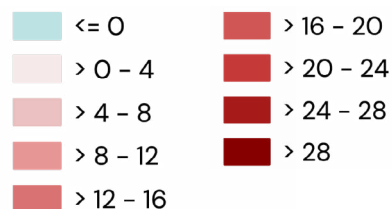
2050 days with maximum temperatures over 95F in 2050: Differences between CMIP6 and CMIP5
