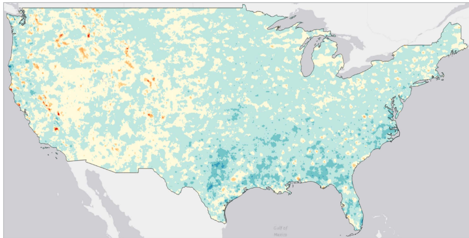
2050 maximum 3-day Precipitation: Difference between CMIP6 and CMIP5 (in mm)
