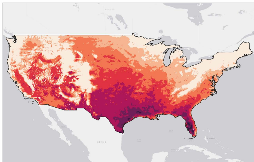
Figure 1: Change in days over 95° F in 2050 compared to historical average 4
