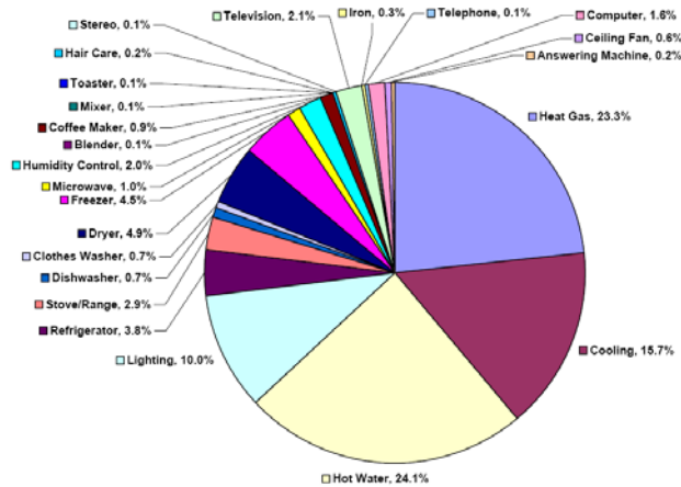
Figure 4. Houston Pie Chart of Baseline Home Energy Use
